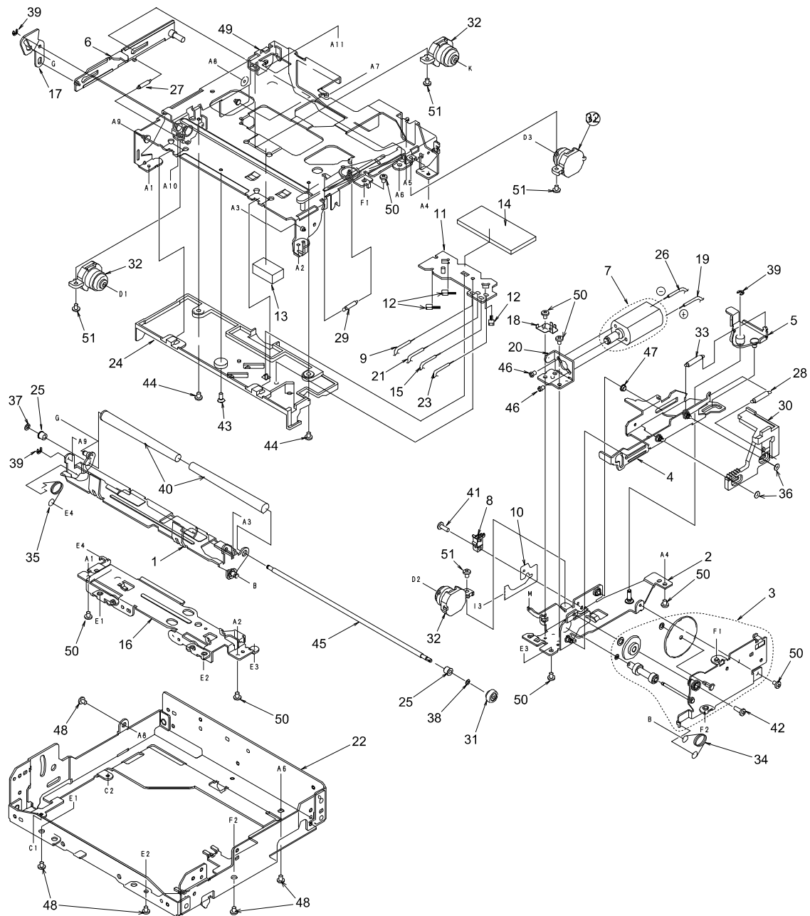
CD mechanism :Mecha chassis section
