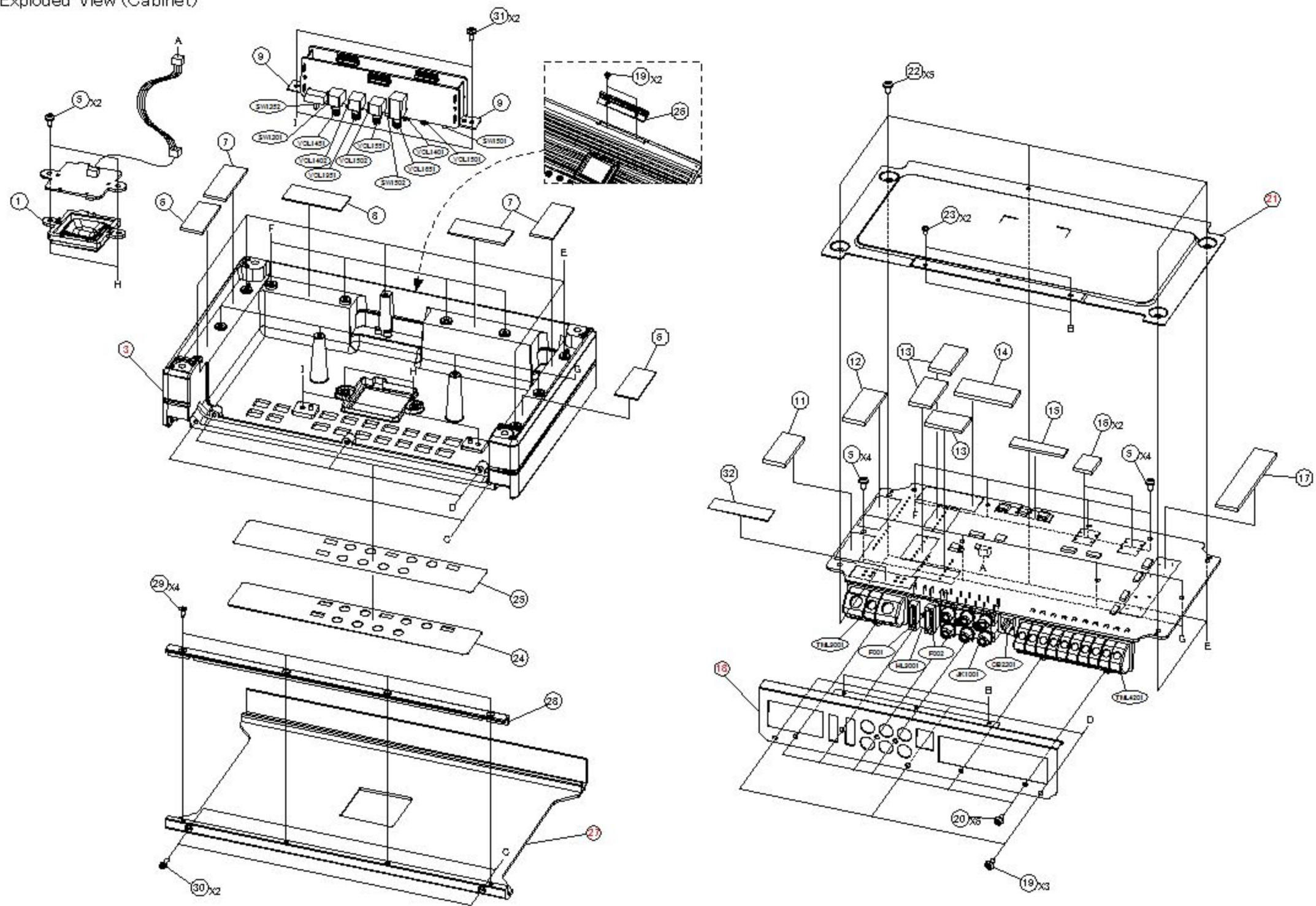
Exploded View (Cabinet)
