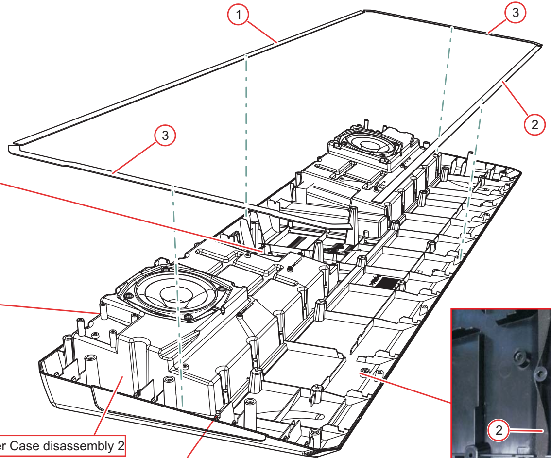
Lower Case disassembly 1
